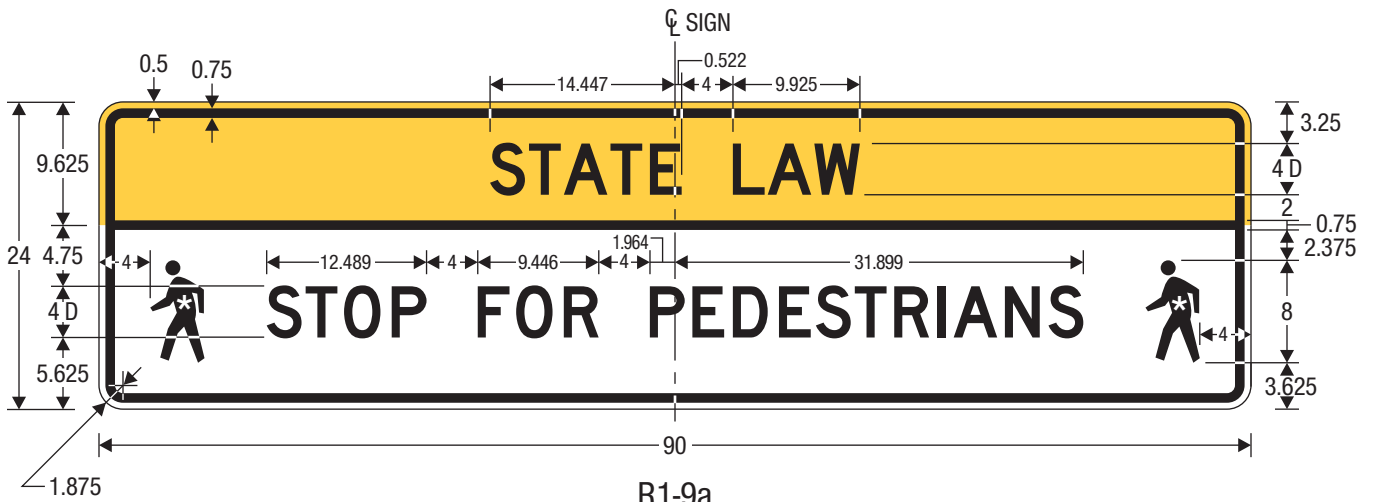
R1-9a OVERHEAD PEDESTRIAN CROSSING (STOP)
