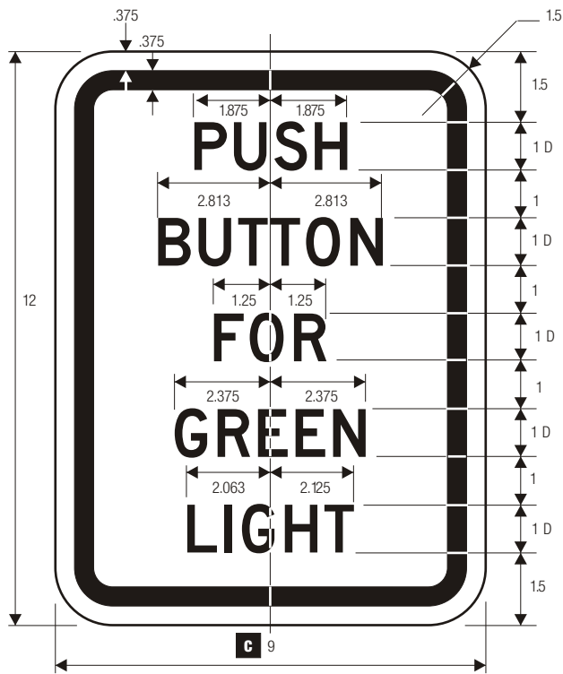
R10-3 PEDESTRIAN TRAFFIC SIGNAL
