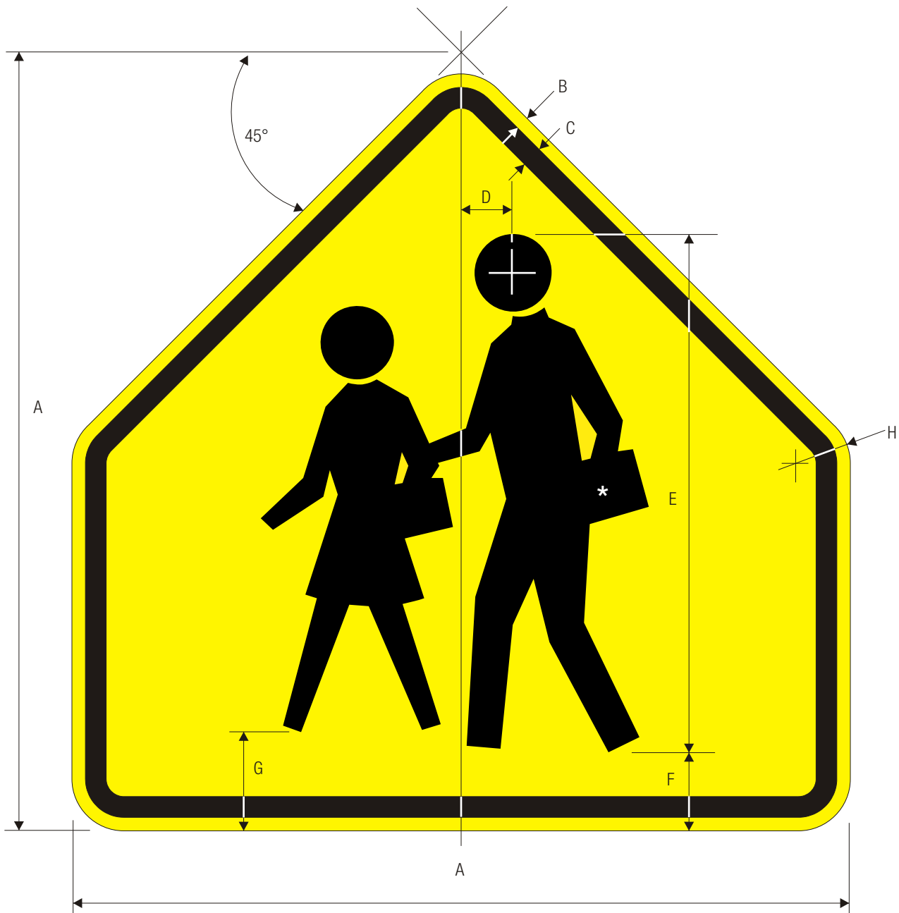
S1-1 SCHOOL
