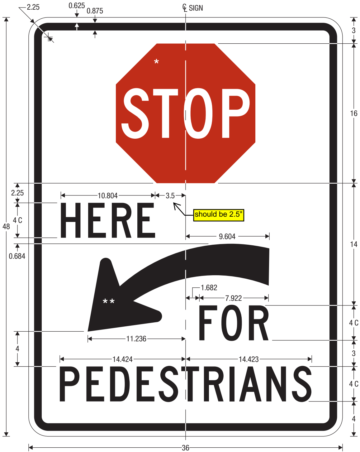
R1-5c STOP HERE FOR PEDESTRIANS (LEFT)
