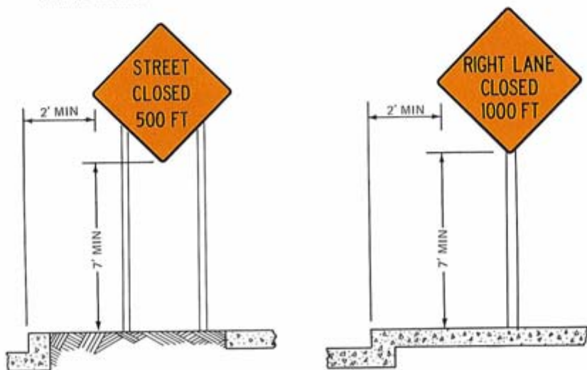
Figure 6-1. Height and lateral locations of signs—typical installation.
