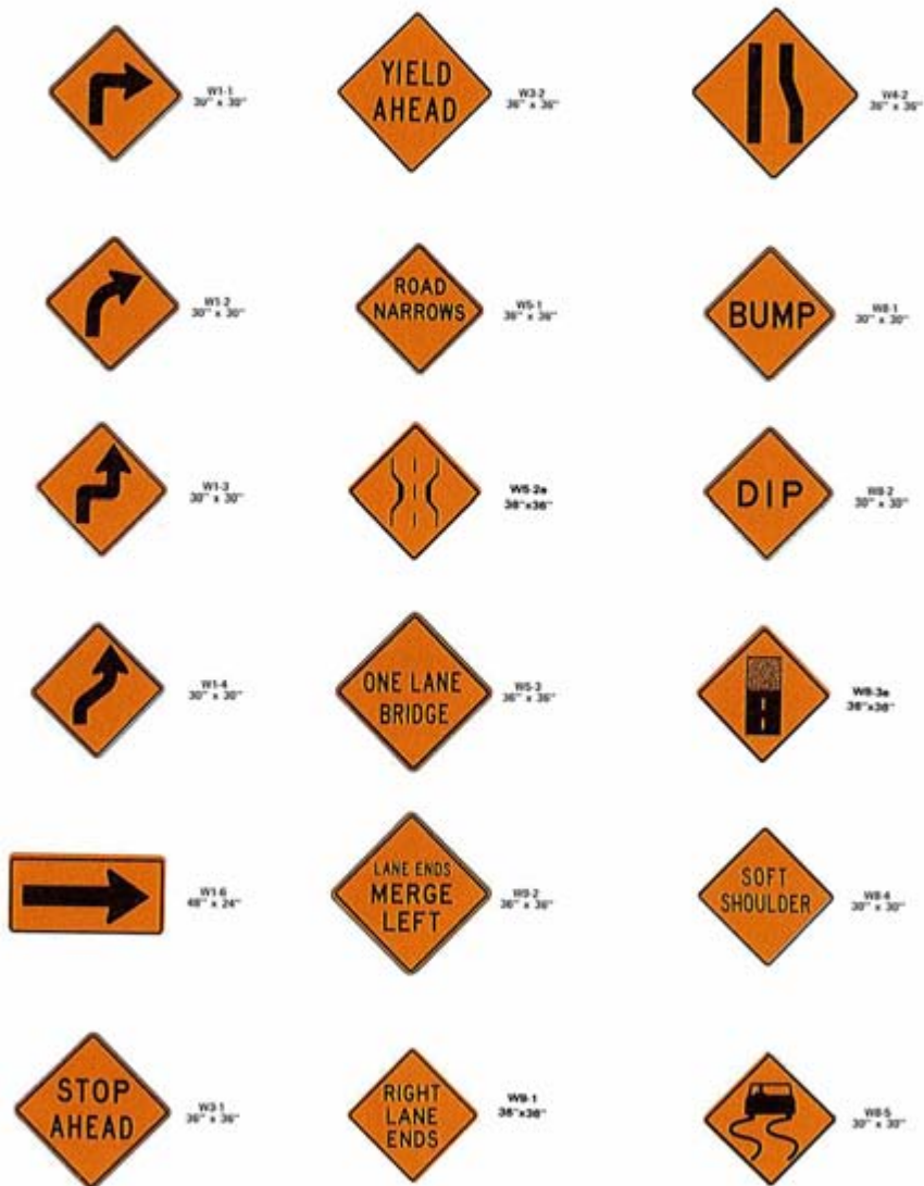
Figure 6-13a. Warning signs used in construction areas.
