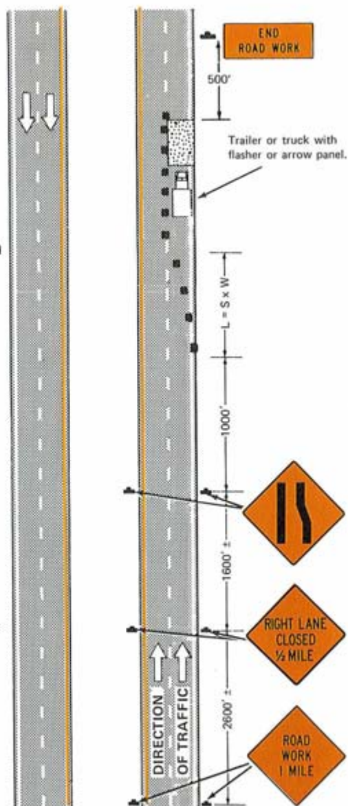
Figure 6-9. Typical application—daytime maintenance operations of short duration on a 4-lane divided roadway where half of roadway is closed.
