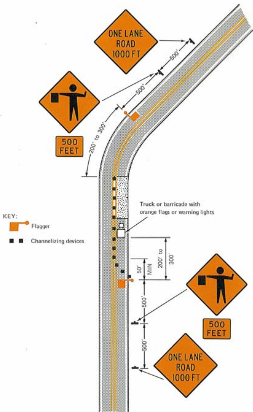
Figure 6-6. Typical application—daytime maintenance operations of short duration on a 2-lane roadway and flagging is provided.
