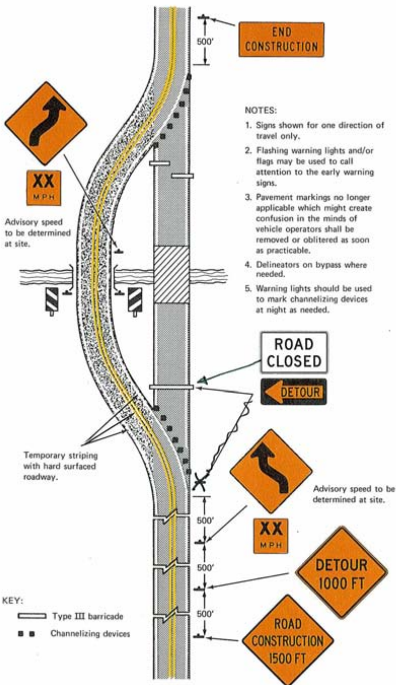
Figure 6-2. Typical applications of traffic control devices on a 2-lane highway where the entire roadway is closed and a bypass detour is provided.
