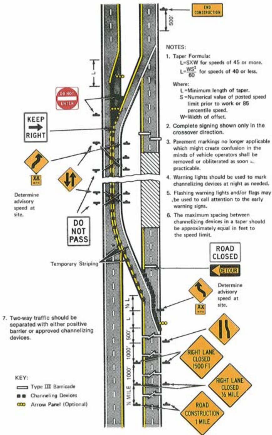
Figure 6-8. Typical application—4-lane divided roadway where one roadway is closed.
